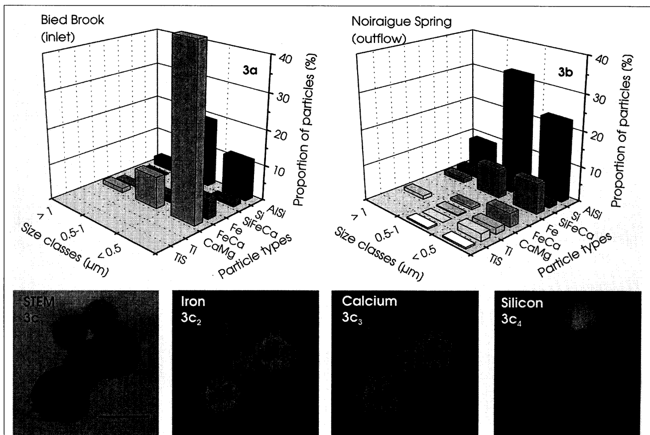
Fig. 3. Size-ordered composition of particles sampled a) in the Bied brook (inlet of the aquifer), and b) in the Noiraigue spring (outflow of the aquifer), and analyzed by STEM-EDS; the labels of particle types express the major elements detected in these particles. c) Micrographs of Fe-Ca-rich particles in the Bied brook (c 1 : STEM; c 2 , c 3 , c 4 : STEM-EDS imaging of Fe, Ca, Si). Scale bars = 0.1 μm.
