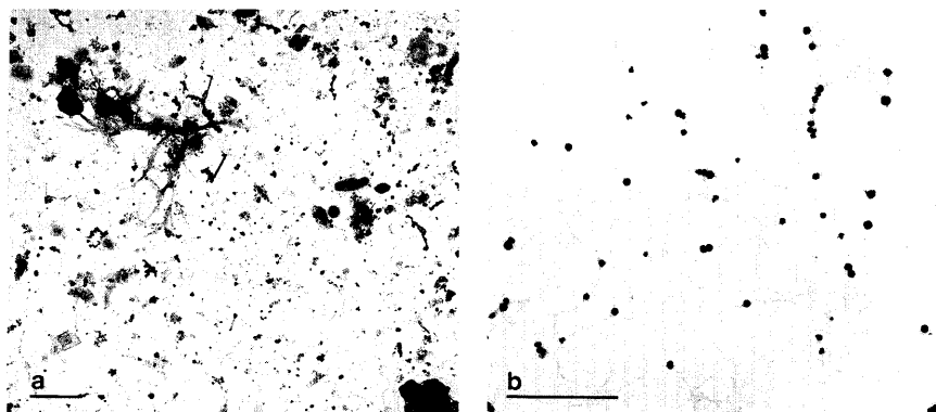
Fig. 4. Micrographs of a) a water sample from the Rhine River, b) a model suspension of hematite micro-particles ( \alpha -Fe 2 O 3 ) and polysaccharide fibrils (xanthan). Scale bars = 1 μm.
