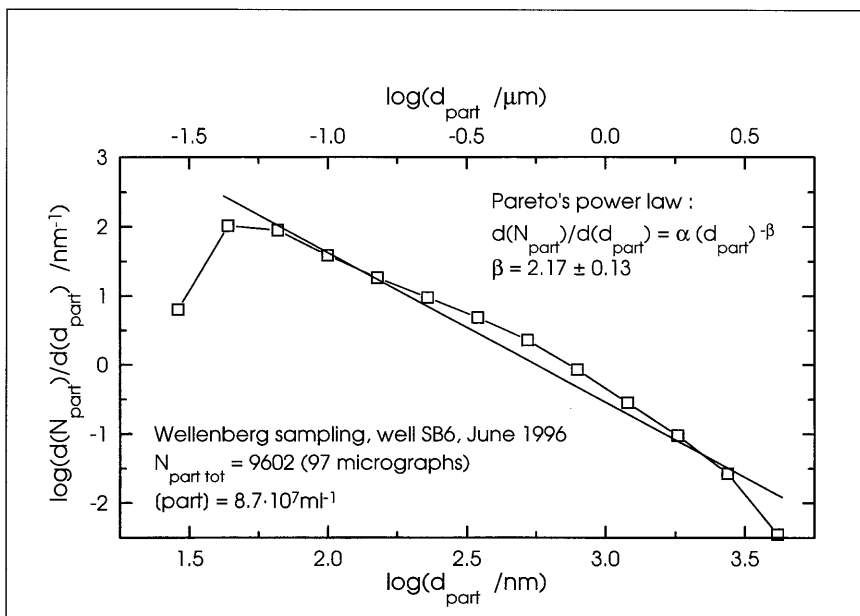
Fig. 2. Particle-size distribution of clay particles sampled in the Wellenberg groundwater and measured by TEM and image analysis. The distribution is expressed according to the Pareto's law: \log(d(N_{part})/d(d_{part})) = f(\log(d_{part})) , with N_{part} = number of particles in a given size interval and d_{part} = diameter of particles. The slope \beta of the power law d(N_{part})/d(d_{part}) = \alpha(d_{part})^{-\beta} is an estimate for the processes of elimination of colloids.
