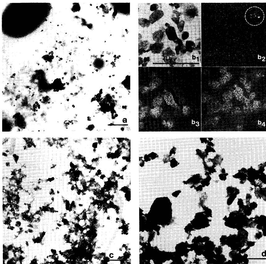
Fig. 1. Micrographs of soil suspensions from a) the O horizon, b) the E horizon (b 1 : TEM; b 2 , b 3 , b 4 : TEM-EELS imaging of Fe-L 2,3 edge, Si-K edge, Al-K edge; note the difference in composition between individual colloids), c) the BP n horizon, and d) the BP n horizon of the podzol in the Arpette valley. Scale bars = 0.5 \mu\text{m} .
