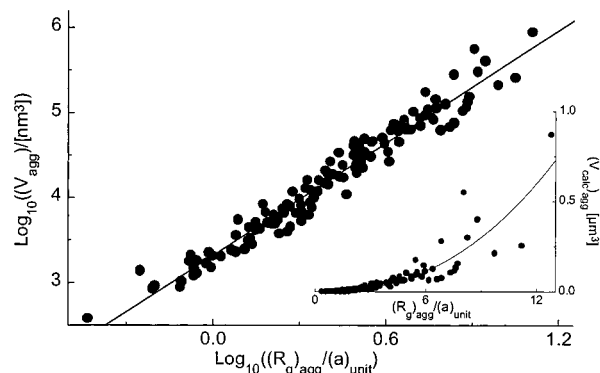
Figure 9. Plot of the volume of \{[\text{Gd}(\text{L}^1)_2]^{5-}\}_n particles and aggregates vs the ratio (radius of gyration of aggregate)/(radius of their elementary units), as determined by image analysis on electron micrographs (128 entities). The inset shows the raw data; the power-law fitting was calculated on the Log–Log representation to minimize the statistical weight of the large (R_g)_{\text{agg}}/(a)_{\text{unit}} on the results.
