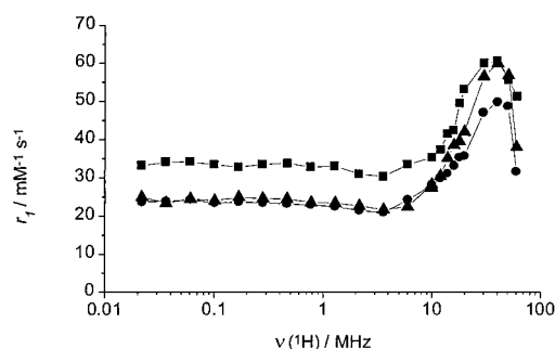
Figure 10. NMRD profiles of \{[\text{Gd}(\text{L}^1)_2]^{5-}\}_n at 5 ( \blacktriangle ), 25 ( \blacksquare ), and 75 ( \bullet ) °C; pH 7.2 (pipes).
